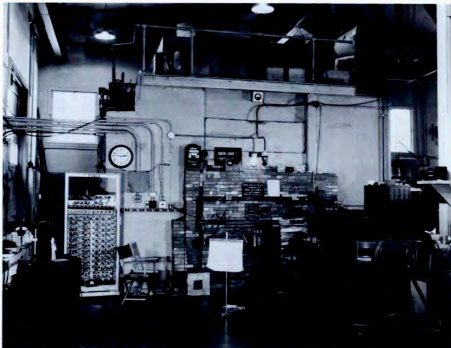
Fig. 2. South face of HYPO, 1948. The plywood boxes on top of the reactor are filled with boron-paraffin for neutron shielding. The device below the clock is the first 100-channel pulse-height analyzer built at Los Alamos.
